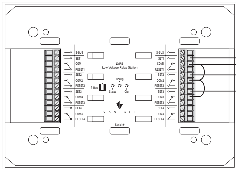
Vantage - Low Voltage Relay System (LVRS)
